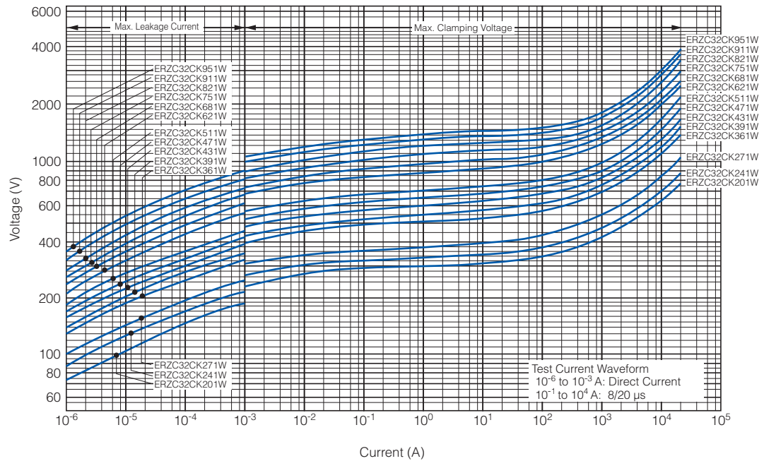
Voltage vs. Current (ERZC32CK201W to ERZC32CK951W)
