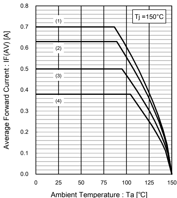
IF(AV) - Ta *2 / Typical Data
