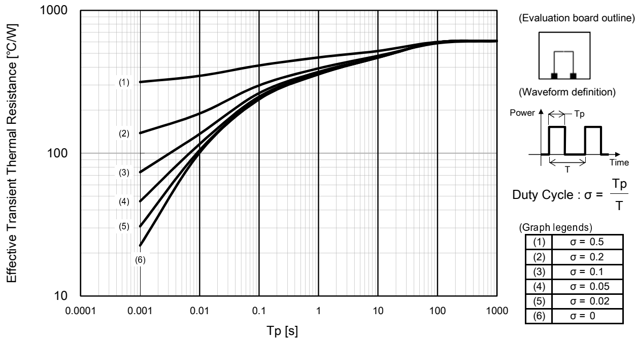
Effective Transient Thermal Resistance - T_p^{*2} / Typical Data
