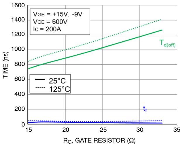
Figure 47. Typical Turn-Off Switching Time vs. R_G
