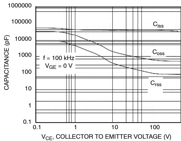
Figure 23. Capacitance
