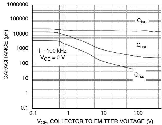
Figure 32. Capacitance
