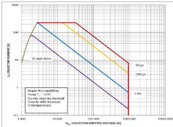
Figure 6. FBSOA
