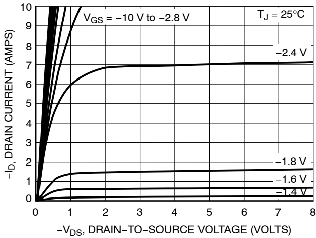
Figure 18. On-Region Characteristics
