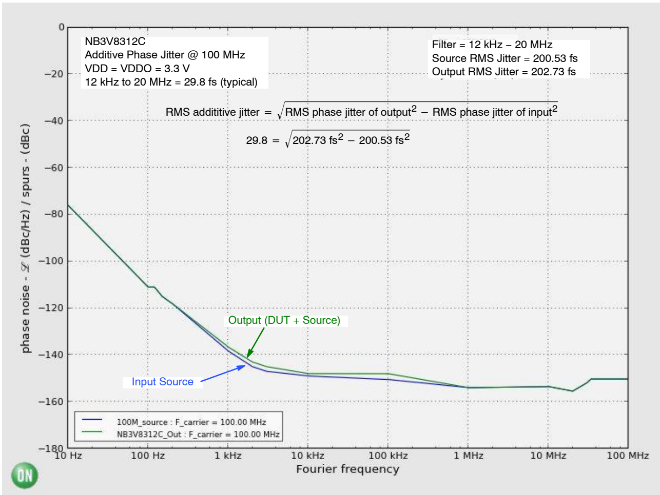
Figure 5. Typical Phase Noise Plot at f_{\text{carrier}} = 100 MHz at an Operating Voltage of 3.3 V, Room Temperature
