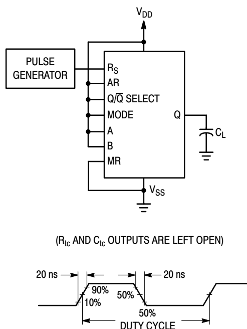
Figure 1. Power Dissipation Test Circuit and Waveform
