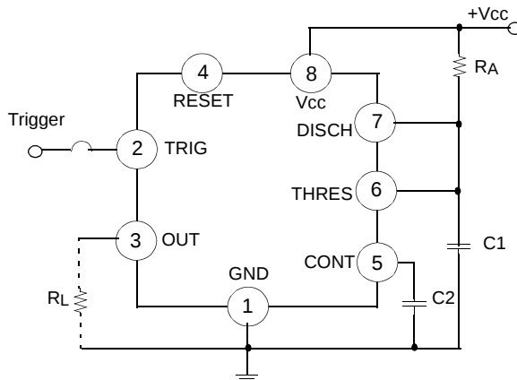
Figure 1. Monoatable Circuit
