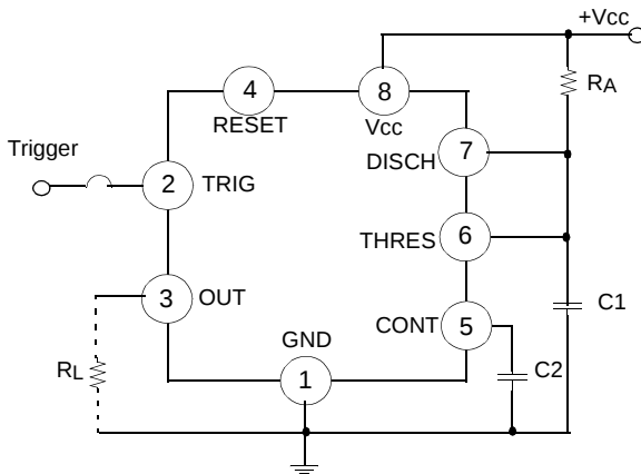
Figure 1. Monoatable Circuit
