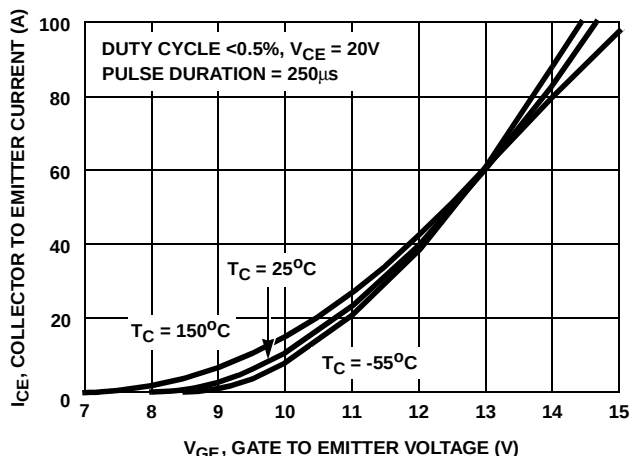
FIGURE 13. TRANSFER CHARACTERISTIC
