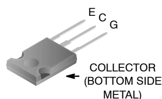
TO-247-3LD SHORT LEAD CASE 340CK JEDEC STYLE
