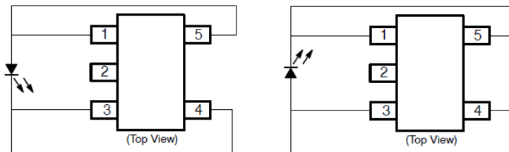
Figure 1. Pin Connections
