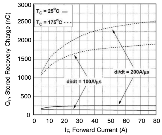
Figure 20. Stored Charge
