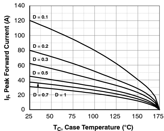
Figure 4. Current Derating
