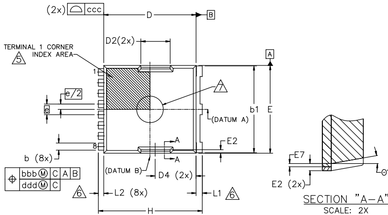
H-PSOF8L 10.38x9.90x2.30, 1.20P CASE 100CU ISSUE G
