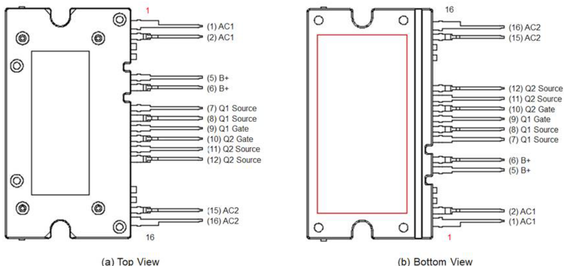
Figure 1. Pin Configuration
