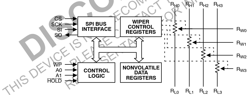
Figure 1. Functional Diagram
