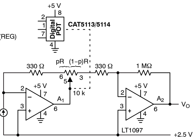
Figure 10. Programmable I to V Converter
