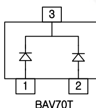
BAV70T
