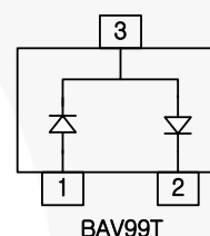
BAV99T
