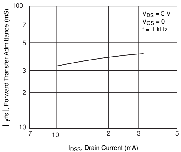
Figure 6. |y_{fs}| - I_D
