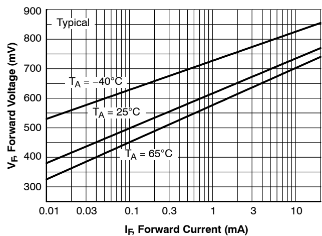
Figure 6. Forward Voltage vs. Ambient Temperature, V_F - 0.01 to 20\ \text{mA} ( -40 to +65^\circ\text{C} )
