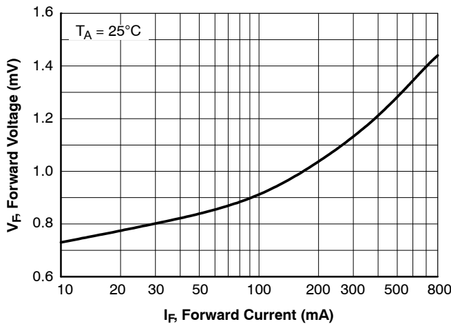
Figure 5. Forward Voltage vs. Forward Current V_F - 10 to 800\ \text{mA}
