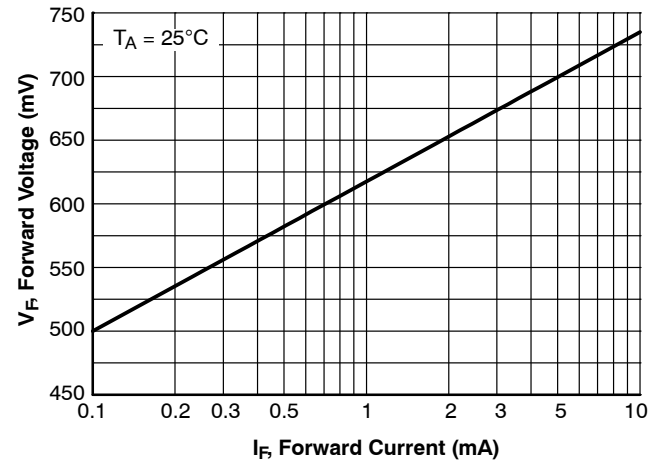
Figure 4. Forward Voltage vs. Forward Current V_F - 0.1 to 10\ \text{mA}
