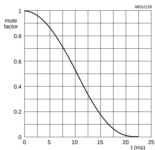
Fig.4 Mute as a function of raised cosine roll-off.
