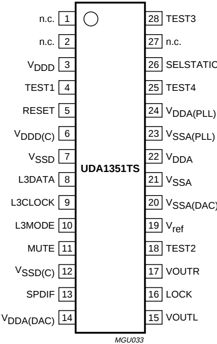
Fig.2 Pin configuration.
