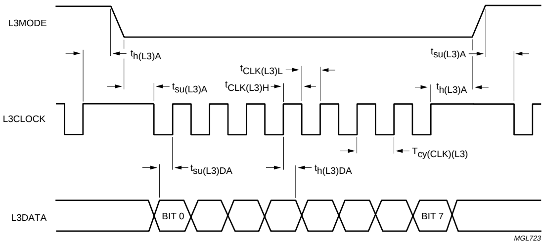
Fig.8 Timing for address mode.
