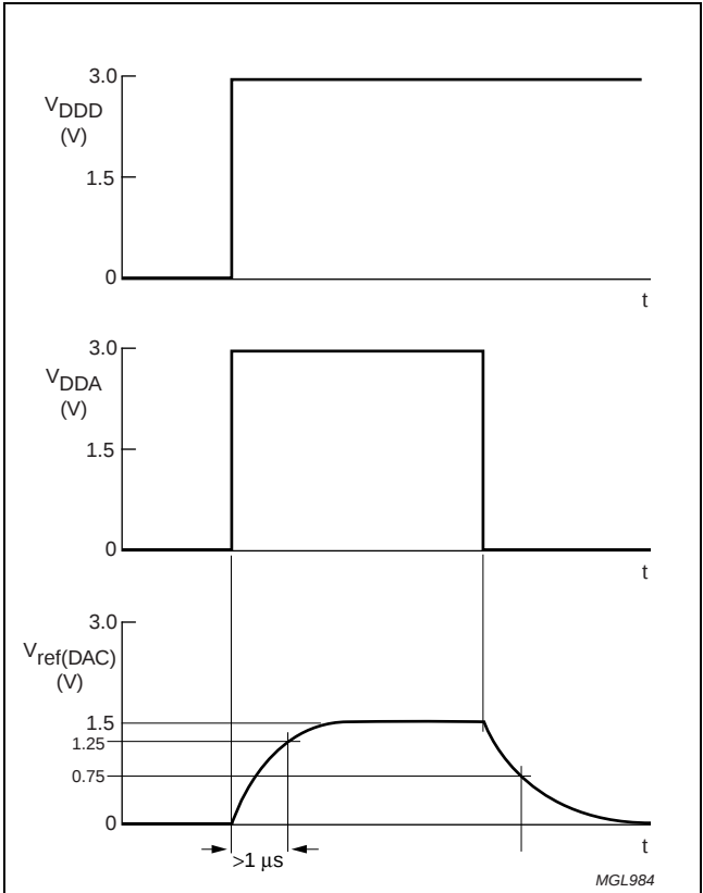
Fig.4 Power-on reset timing.
