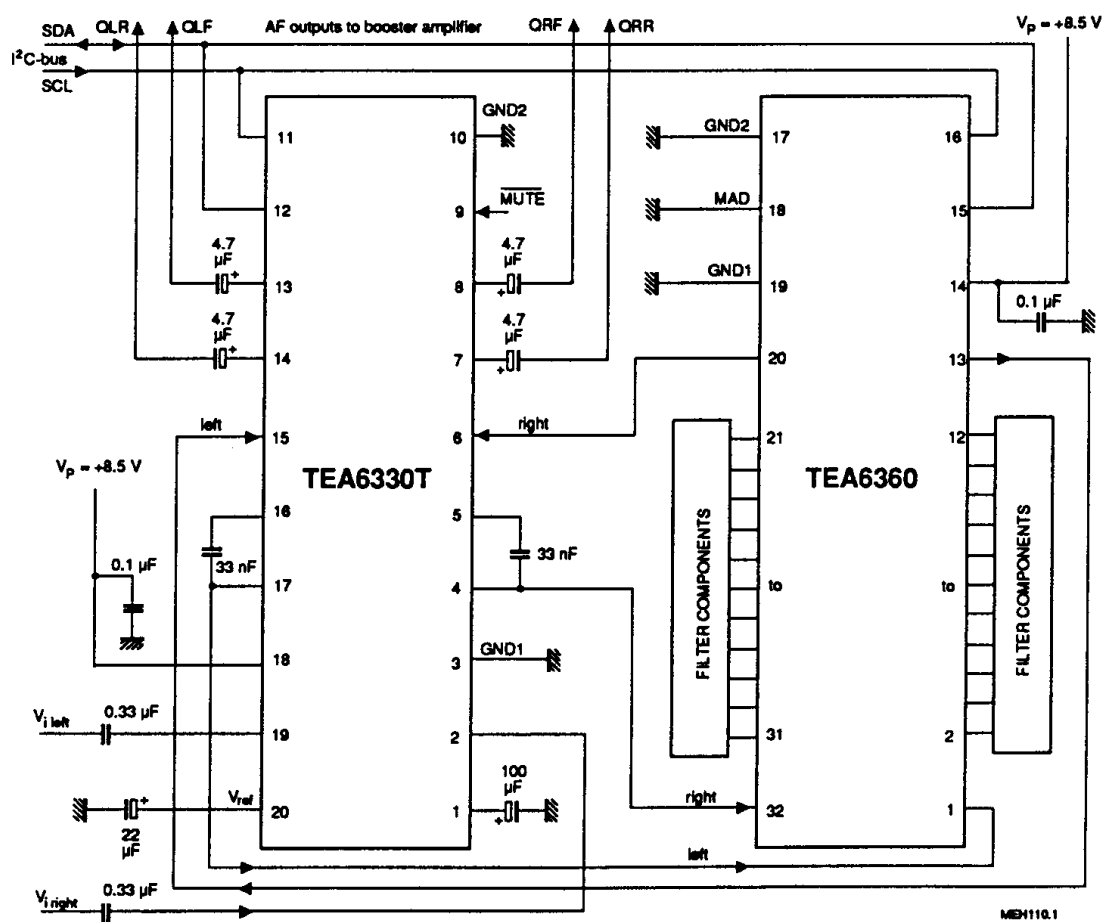
Fig.4 Application for car radio ( V_p < 8.5 V).
