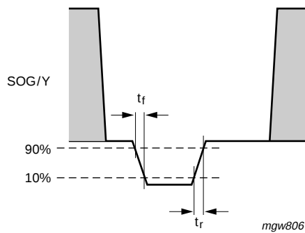
Fig 9. Horizontal sync pulse on SOG/Y
