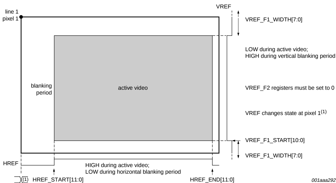
Fig 6. HREF and VREF in progressive case
