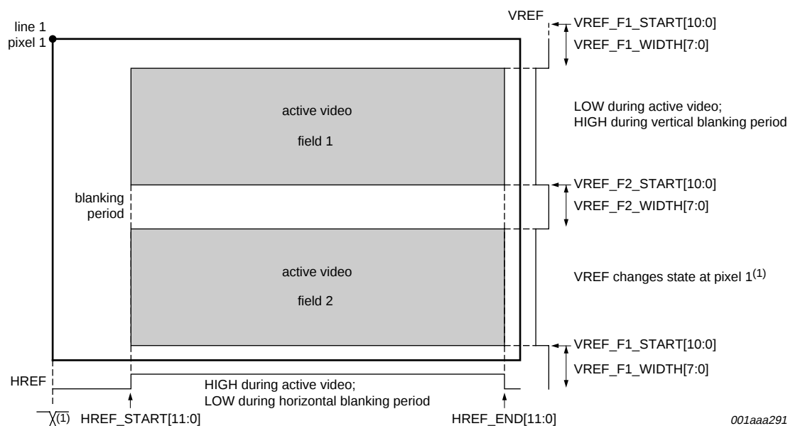
Fig 5. HREF and VREF in interlaced case
