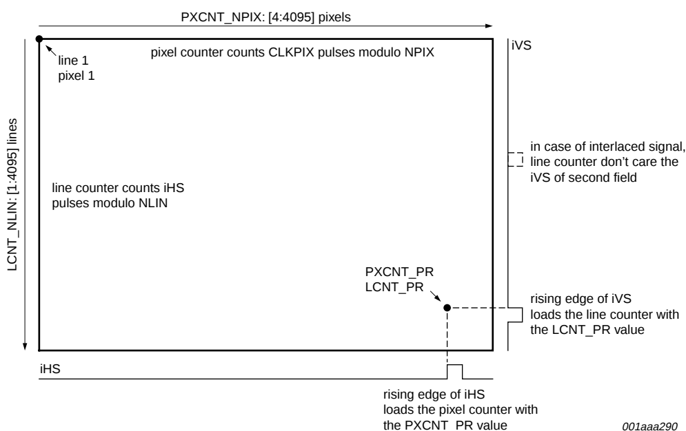
Fig 4. Line and pixel counters
