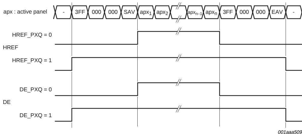
Fig 8. Pixel qualification
