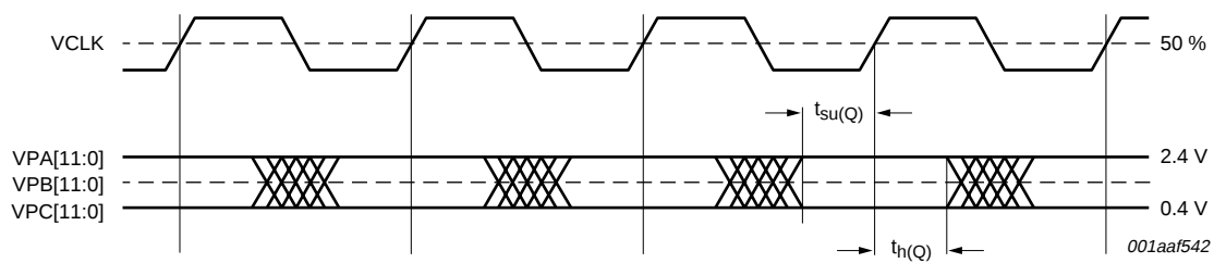
Fig 10. Output timing
