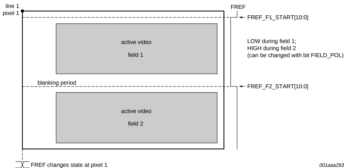
Fig 7. FREF in interlaced case
