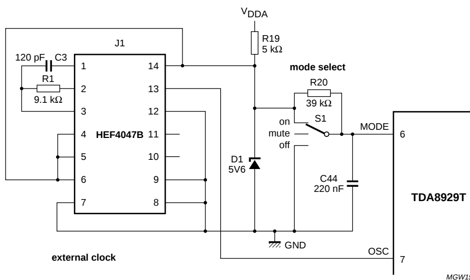
Fig.11 External oscillator circuit.
