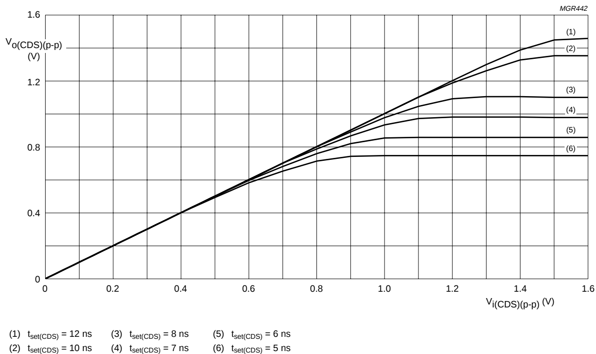
Fig.14 CDS output.
