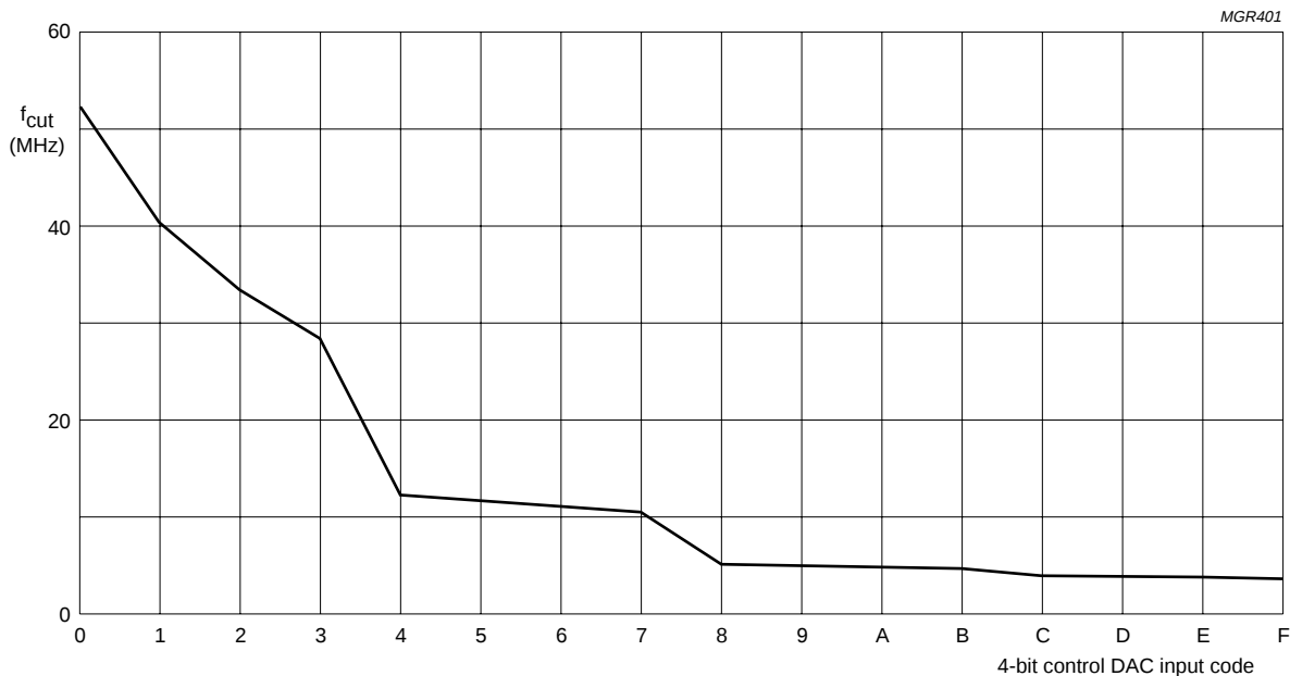
Fig.13 AGC bandwidth.
