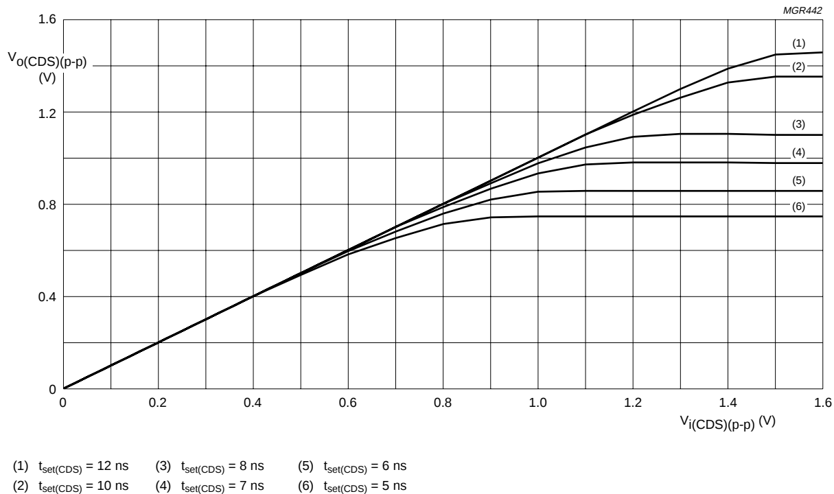
Fig.14 CDS output.
