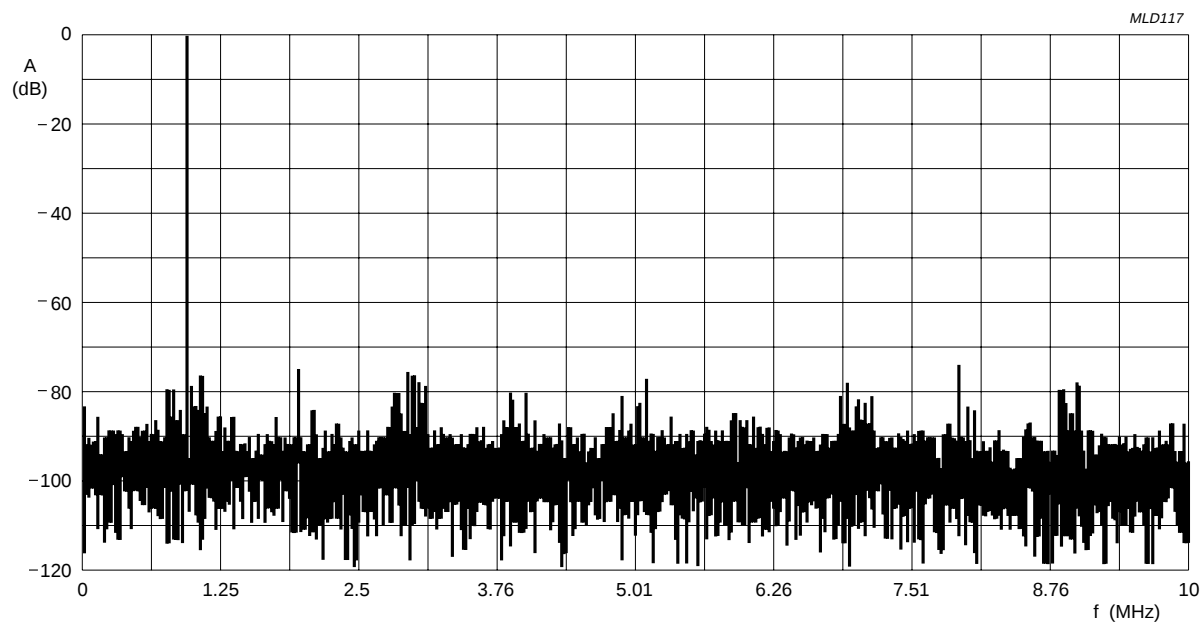
Fig.9 Typical fast Fourier transform ( f_{\text{clk}} = 20 \text{ MHz} ; f_i = 1 \text{ MHz} ).
