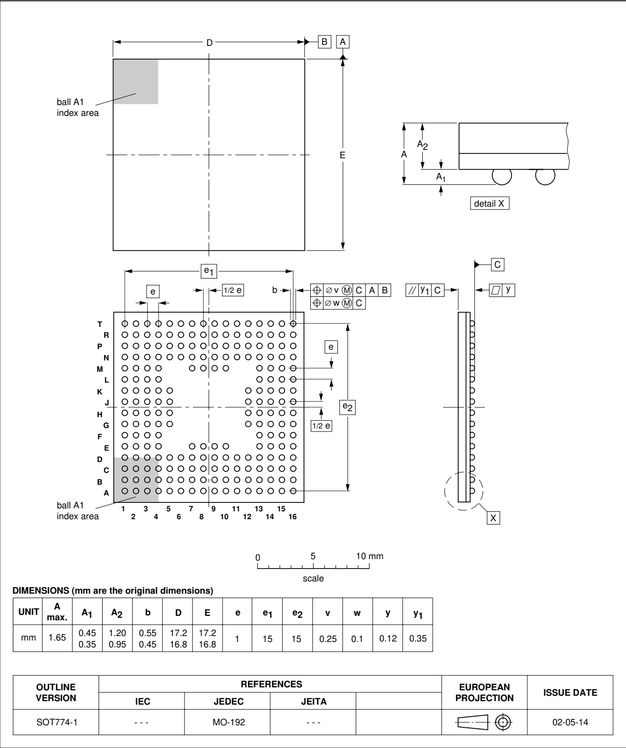
Fig 12. Package outline SOT774-1 (LBGA208)
