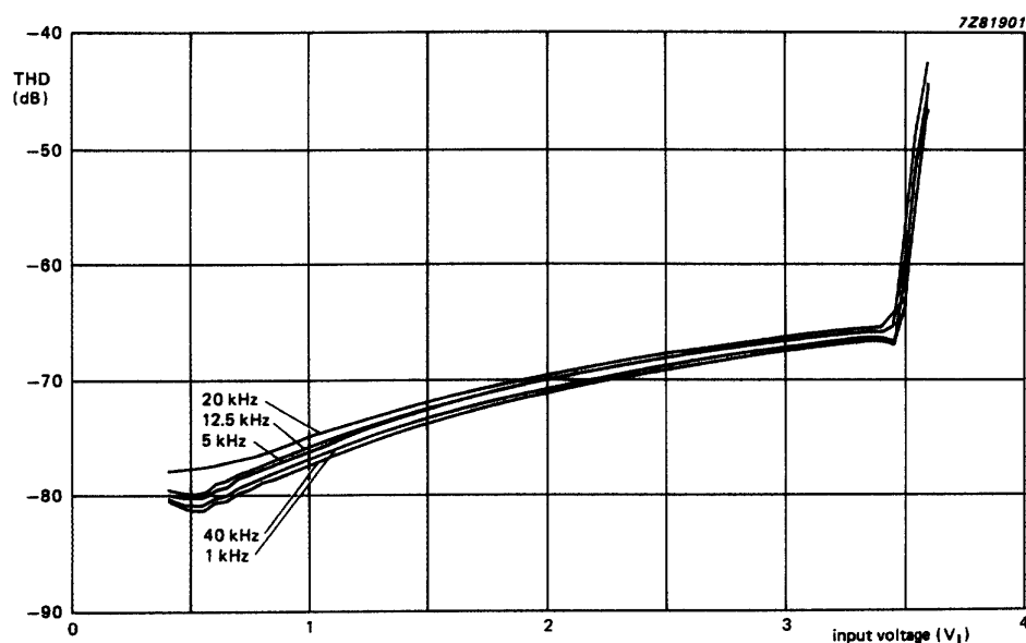
Fig.8 Input signal handling capability; gain = -10 dB; R_S = 600 \Omega ; R_L = 10 \text{ k}\Omega ; bass/treble = 0 dB; V_{CC} = 12 \text{ V} .
