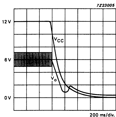
Fig.20 Turn-off behaviour; with modulation (shaded area).
