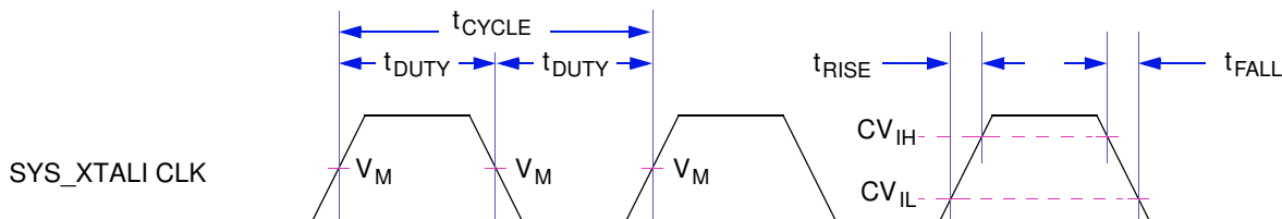
Figure 3. Timing Diagram—SYS_XTALI
