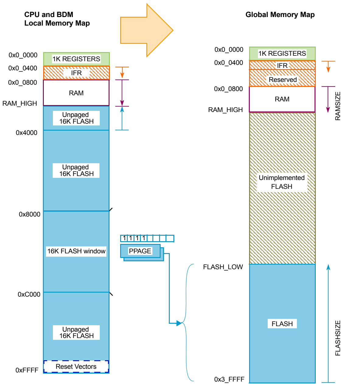
Figure 45. MC9S12I32 Global Address Mapping
