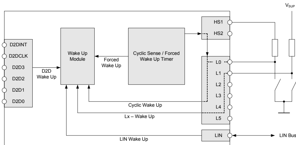
Figure 19. Wake-up Sources
