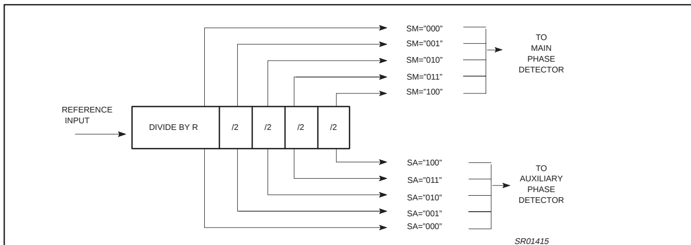
Figure 6. Reference Divider
