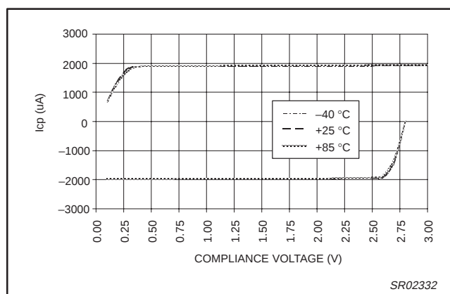
Figure 14. PHI Charge Pump Output vs. Temperature (CP = 01_12x; V_{DD} = 3.0 V; I_{SET} = 164 \mu A)
