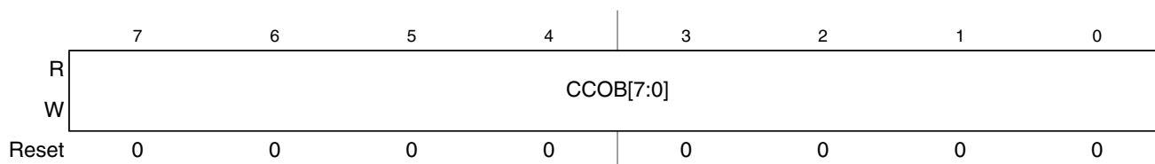
Figure 17-16. Flash Common Command Object Low Register (FCCOBLO)
