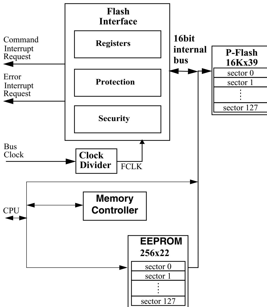
Figure 17-1. FTMRG64K512 Block Diagram
