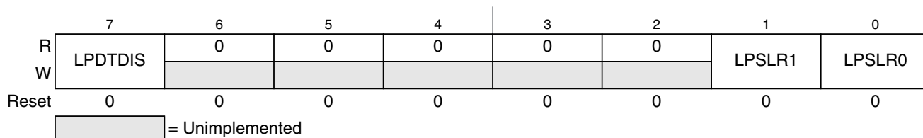
Figure 15-6. LIN Slew Rate Mode Register (LPSLRM)
