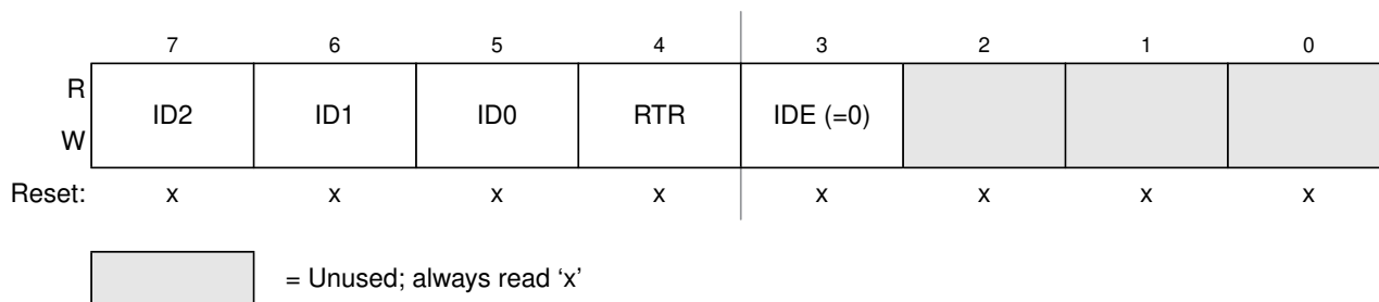
Figure 8-31. Identifier Register 1 — Standard Mapping
