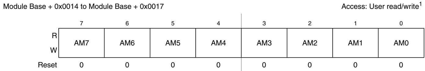
Figure 18-22. MSCAN Identifier Mask Registers (First Bank) — CANIDMR0–CANIDMR3
