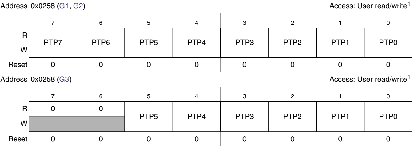
Figure 2-35. Port P Data Register (PTP)
