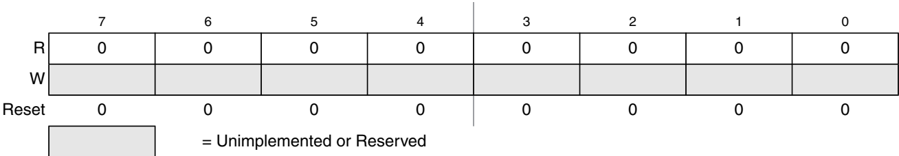
Figure 26-24. Flash Reserved6 Register (FRSV6)
