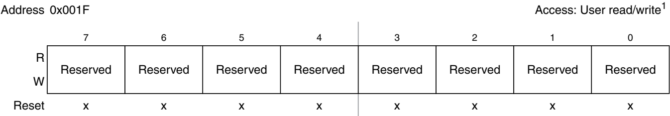
Figure 2-15. Reserved Register
