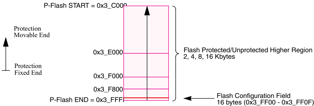
Figure 24-2. P-Flash Memory Map
