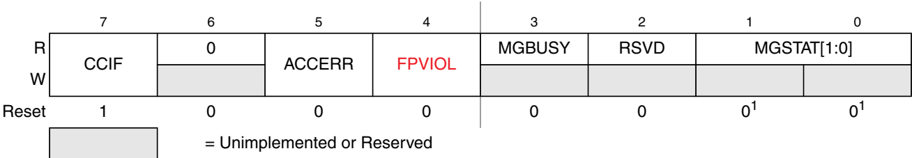
Figure 27-11. Flash Status Register (FSTAT)
