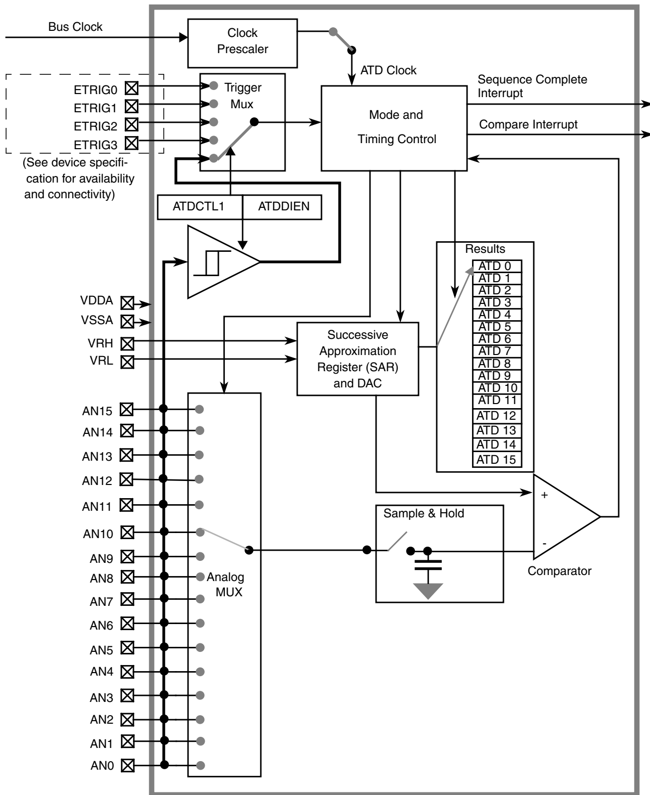
Figure 15-1. ADC10B16C Block Diagram
