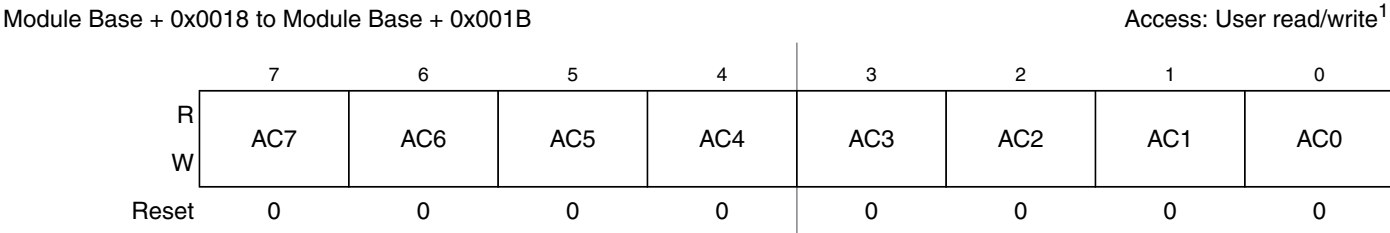
Figure 18-21. MSCAN Identifier Acceptance Registers (Second Bank) — CANIDAR4–CANIDAR7
