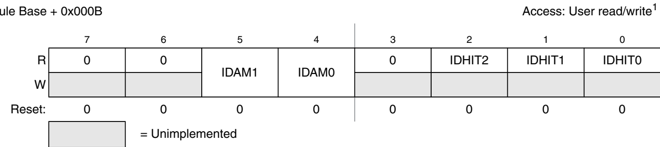
Figure 18-15. MSCAN Identifier Acceptance Control Register (CANIDAC)
