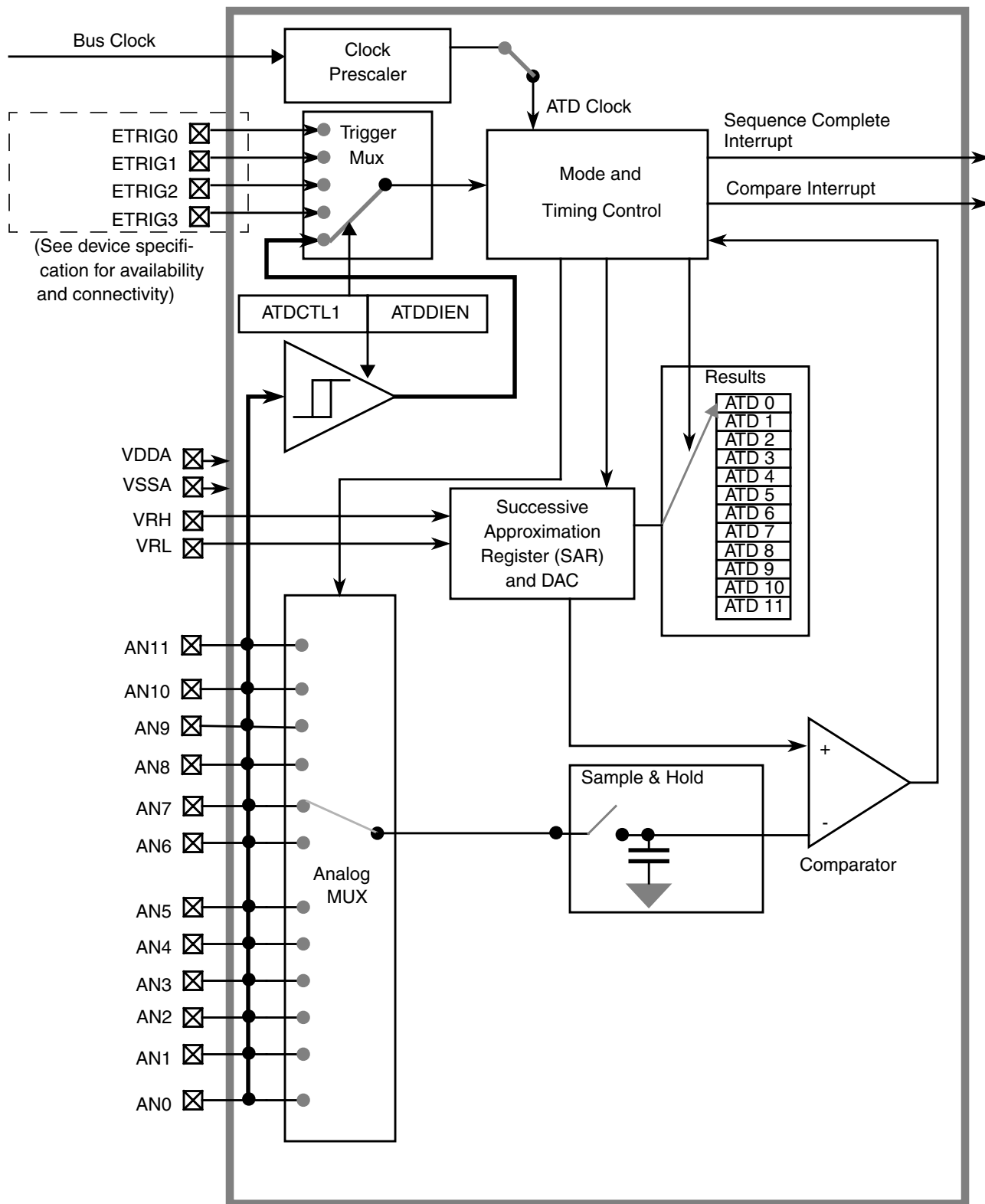
Figure 14-1. ADC12B12C Block Diagram
