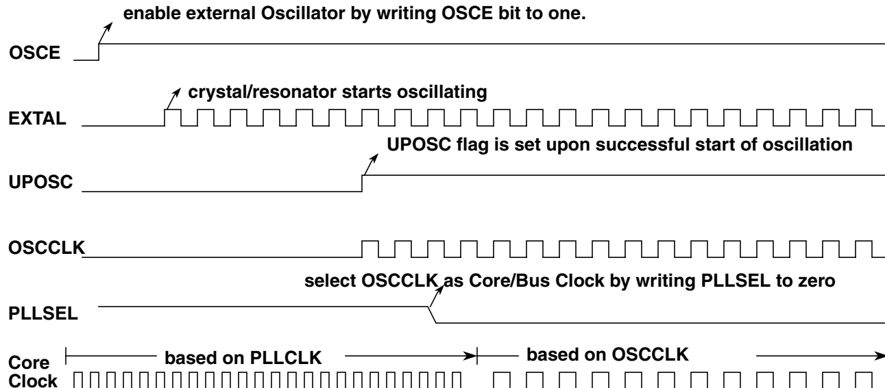
Figure 10-33. Enabling the External Oscillator
