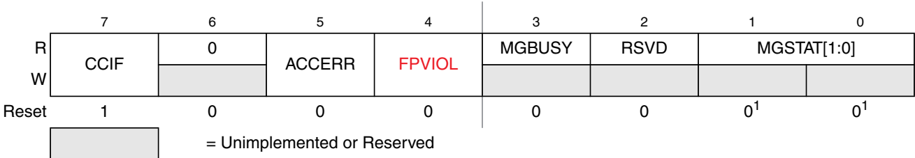
Figure 28-11. Flash Status Register (FSTAT)
