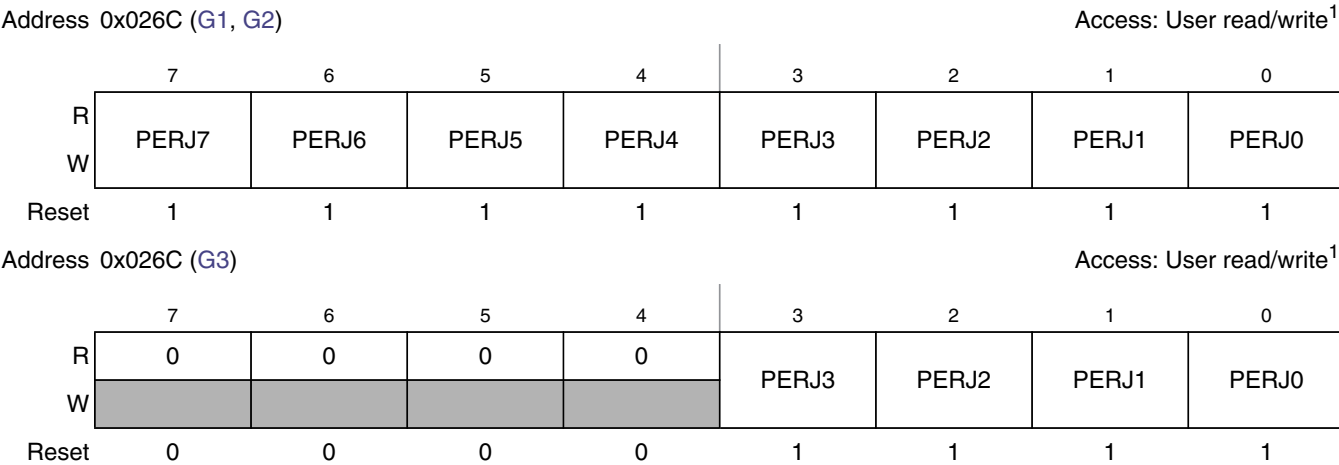
Figure 2-45. Port J Pull Device Enable Register (PERJ)
