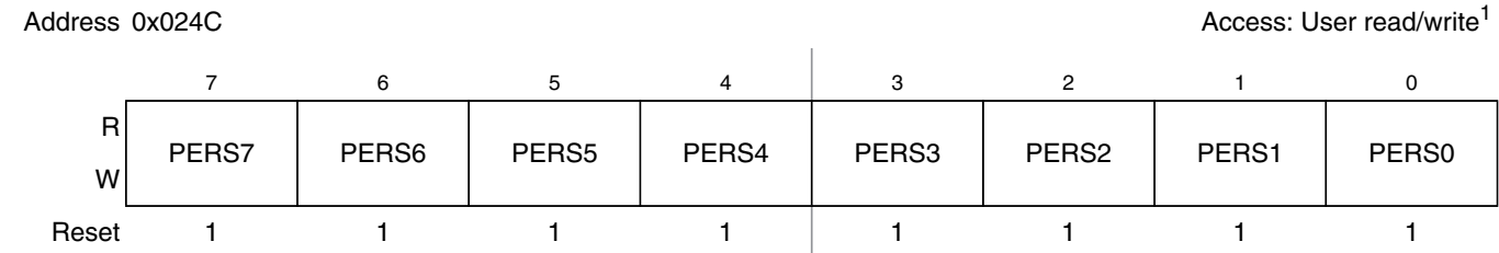
Figure 2-24. Port S Pull Device Enable Register (PERS)
