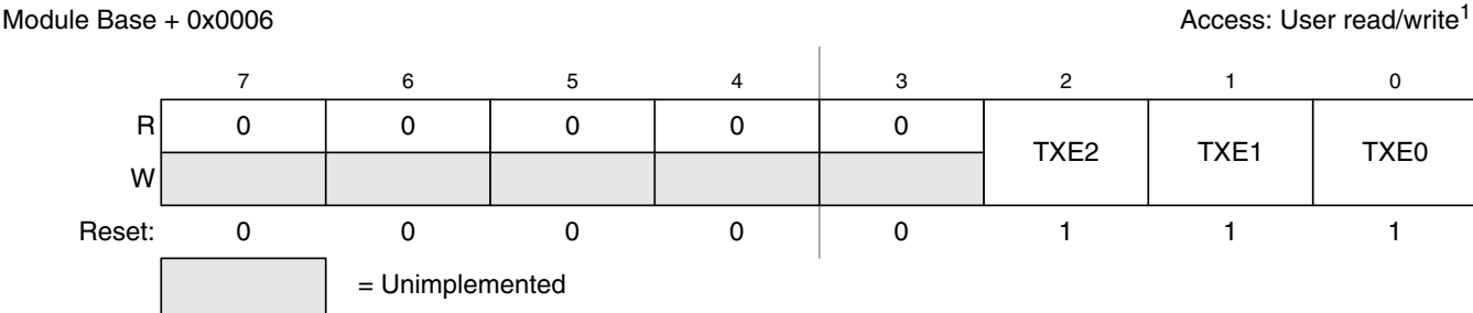
Figure 18-10. MSCAN Transmitter Flag Register (CANTFLG)
