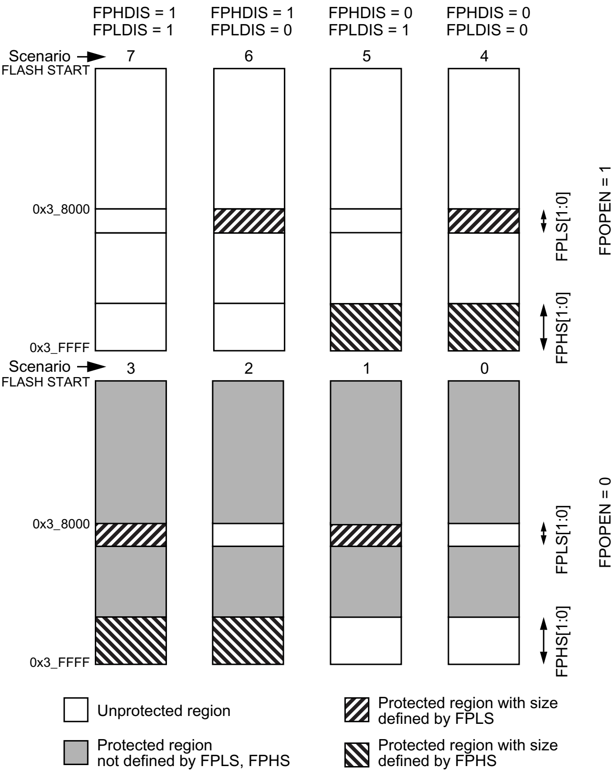
Figure 30-14. P-Flash Protection Scenarios
