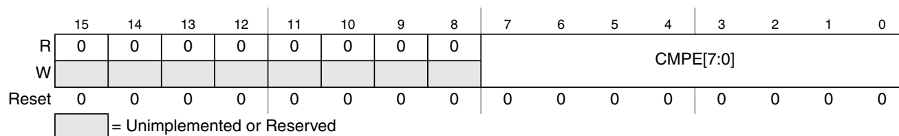
Figure 12-10. ATD Compare Enable Register (ATDCMPE)
