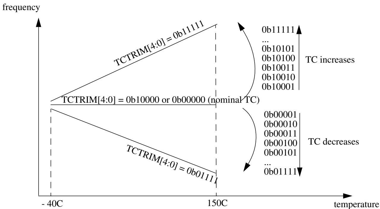
Figure 10-26. Influence of TCTRIM[4:0] on the Temperature Coefficient
