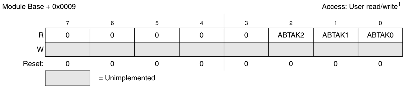
Figure 18-13. MSCAN Transmitter Message Abort Acknowledge Register (CANTAABK)
