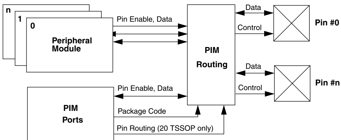
Figure 2-1. Block Diagram
