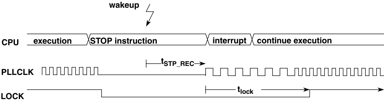
Figure 10-31. Stop Mode using PLLCLK as Bus Clock
