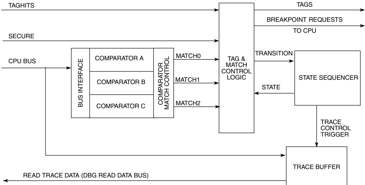
Figure 8-23. DBG Overview
