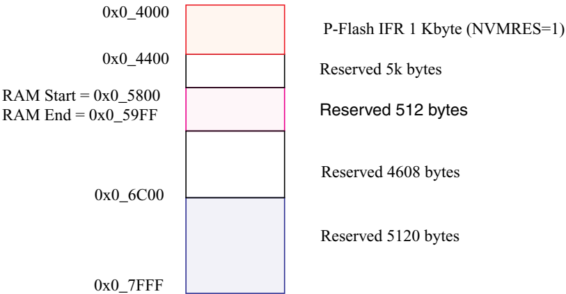
Figure 24-3. Memory Controller Resource Memory Map (NVMRES=1)
