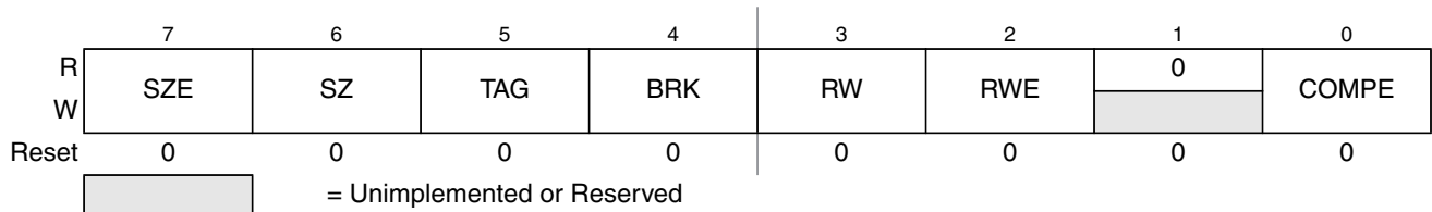
Figure 8-14. Debug Comparator Control Register DBGBCTL (Comparator B)
