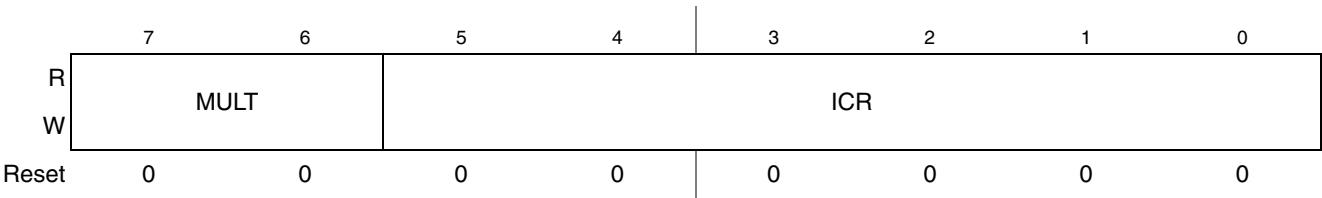
Figure 11-4. IIC Frequency Divider Register (IICF)
