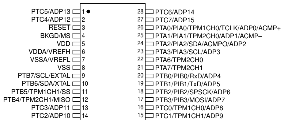
Figure 2-1. 28-Pin TSSOP
