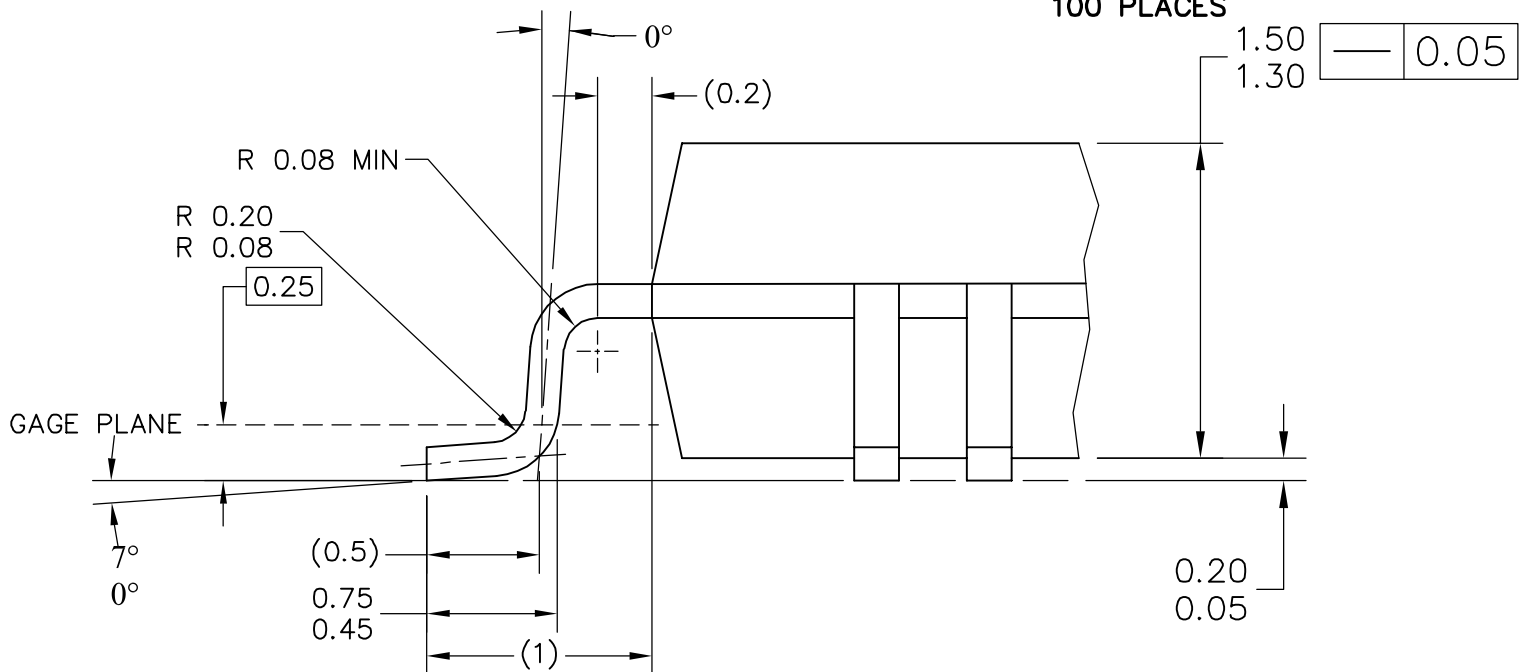
VIEW B
