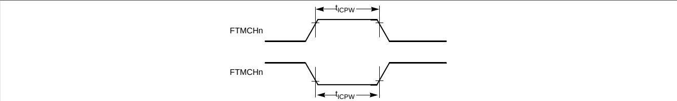
Figure 12. Timer input capture pulse
