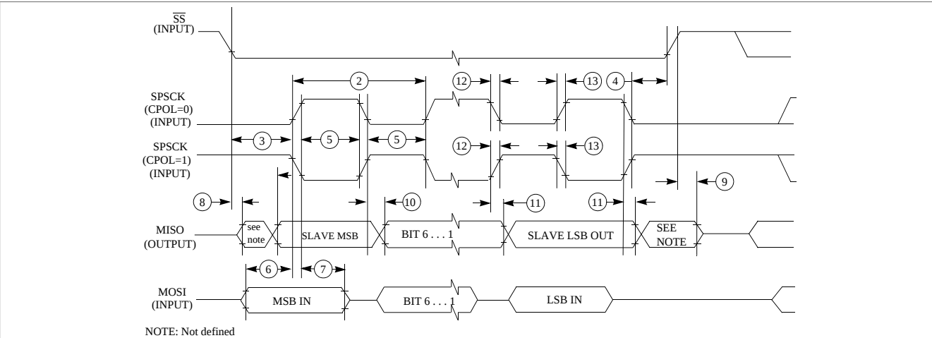
Figure 19. SPI slave mode timing (CPHA = 0)
