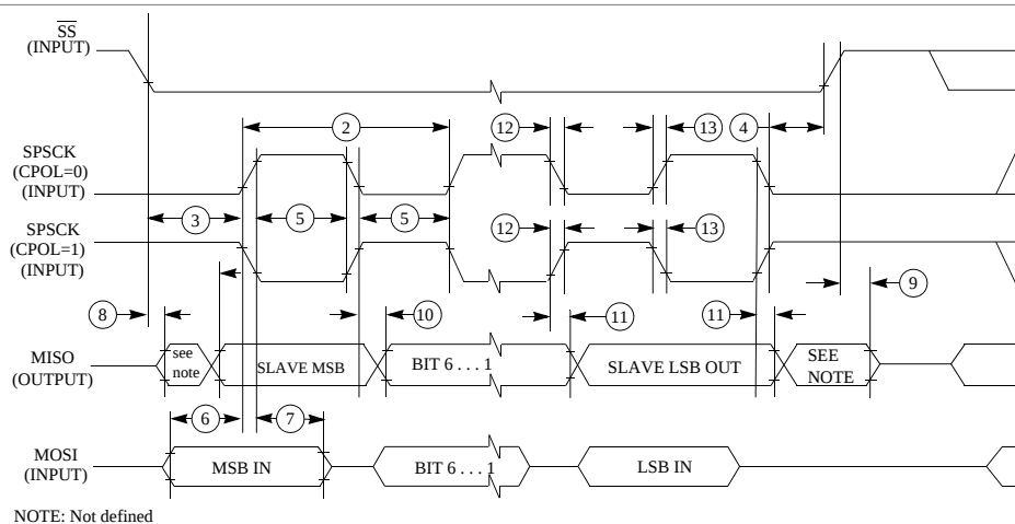
Figure 19. SPI slave mode timing (CPHA = 0)
