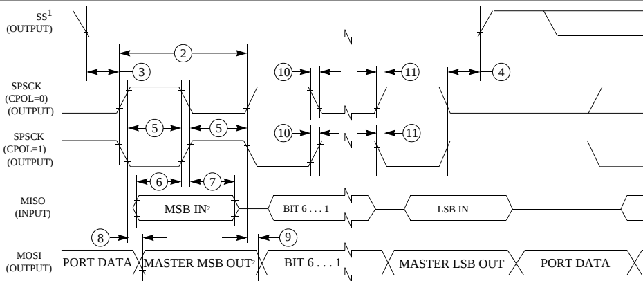
Figure 17. SPI master mode timing (CPHA=0)
