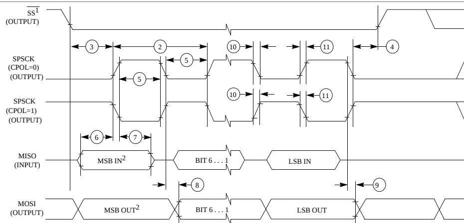
Figure 17. SPI master mode timing (CPHA=0)
