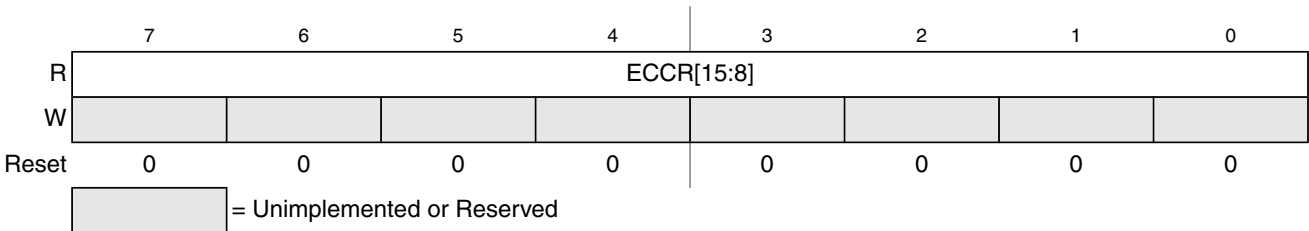
Figure 25-20. Flash ECC Error Results High Register (FECCRHI)
