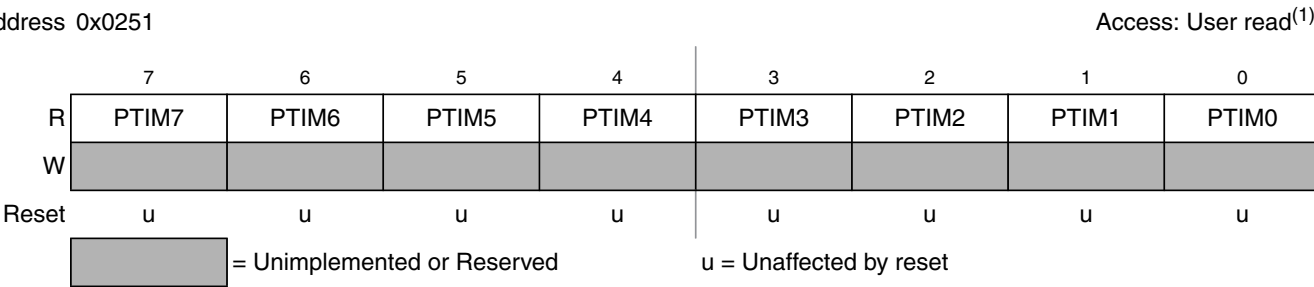
Figure 2-36. Port M Input Register (PTIM)
