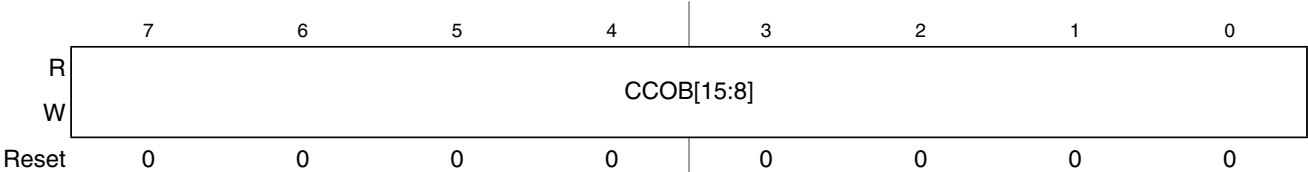
Figure 27-16. Flash Common Command Object High Register (FCCOBHI)
