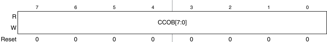
Figure 24-17. Flash Common Command Object Low Register (FCCOBLO)
