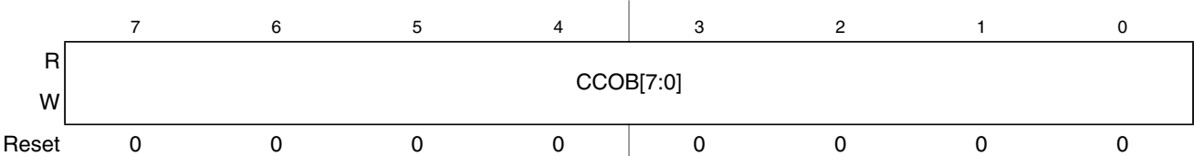
Figure 27-17. Flash Common Command Object Low Register (FCCOBLO)
