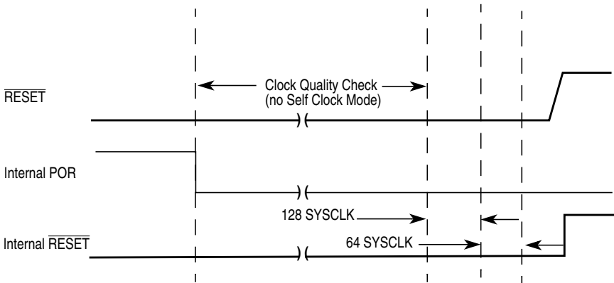
Figure 11-23. \overline{\text{RESET}} Pin Held Low Externally
