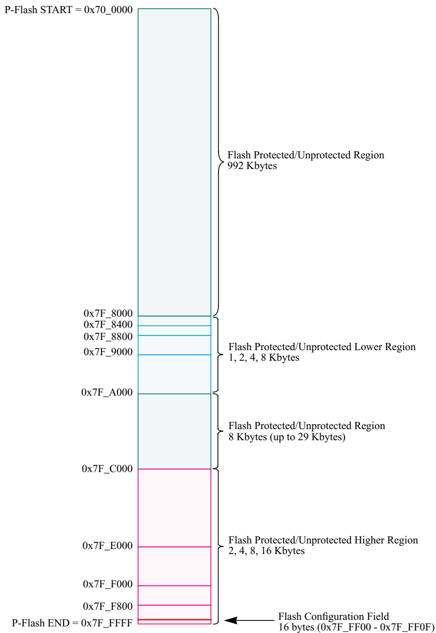
Figure 29-2. P-Flash Memory Map
