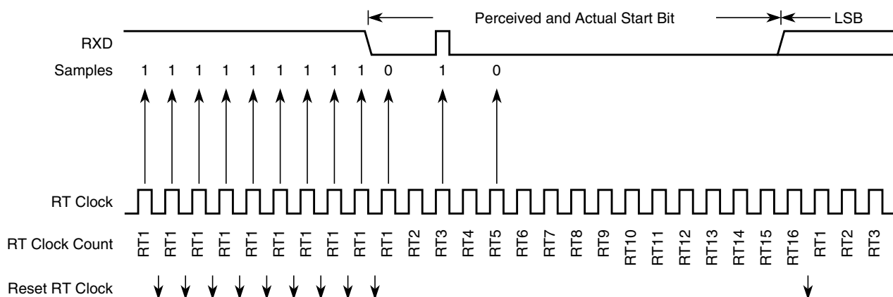
Figure 20-25. Start Bit Search Example 4
