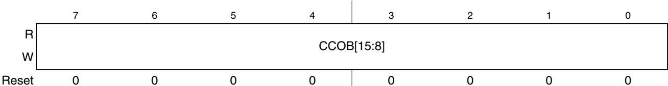
Figure 24-16. Flash Common Command Object High Register (FCCOBHI)
