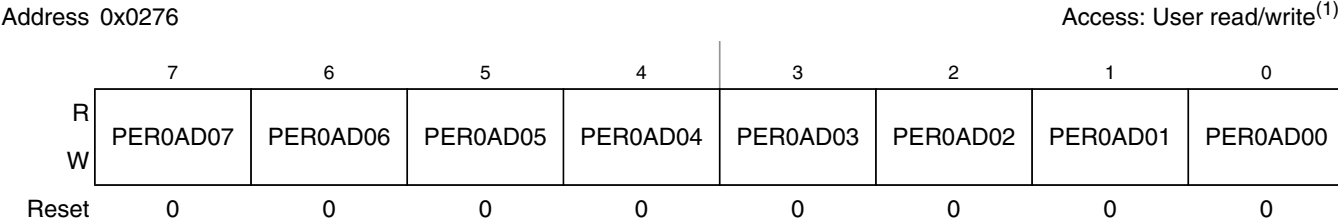
Figure 2-73. Port AD0 Pull Device Up Register 0 (PER0AD0)
