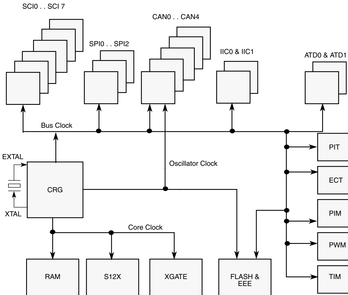
Figure 1-9. Clock Connections
