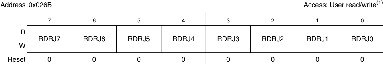
Figure 2-62. Port J Reduced Drive Register (RDRJ)
