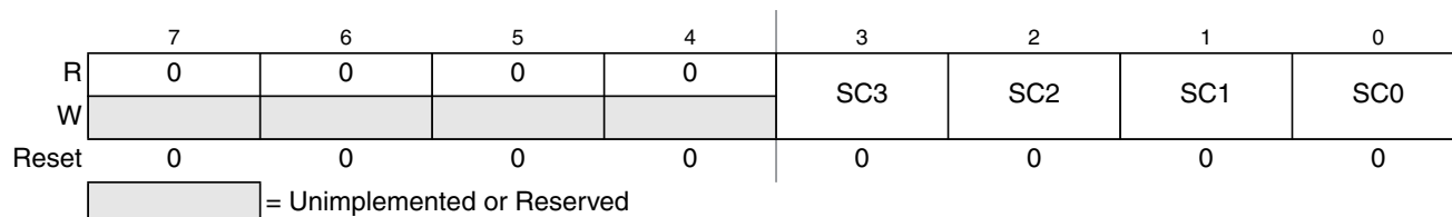
Figure 8-10. Debug State Control Register 2 (DBGSCR2)
