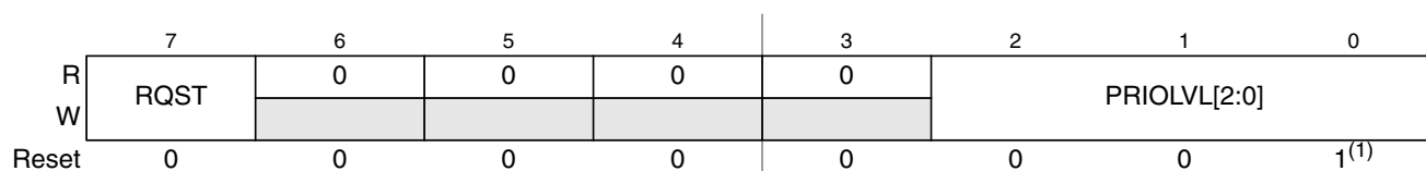
Figure 6-8. Interrupt Request Configuration Data Register 2 (INT_CFDATA2)
