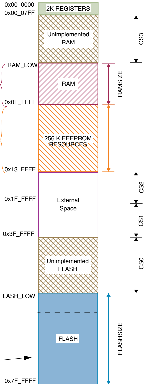
Figure 1-2. MC9S12XE100 Global Memory Map
