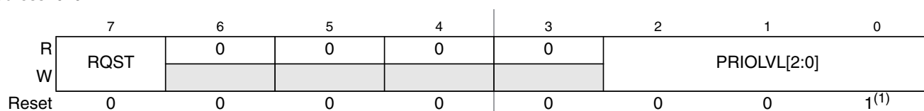
Figure 6-9. Interrupt Request Configuration Data Register 3 (INT_CFDATA3)
