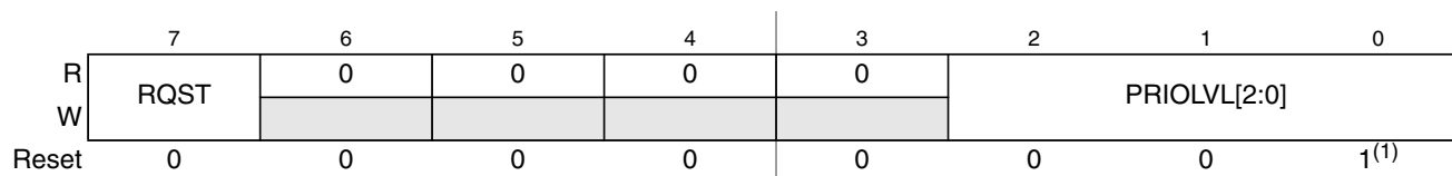
Figure 6-6. Interrupt Request Configuration Data Register 0 (INT_CFDATA0)
