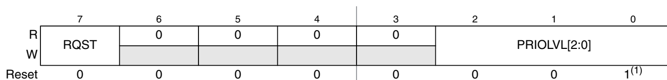
Figure 6-7. Interrupt Request Configuration Data Register 1 (INT_CFDATA1)
