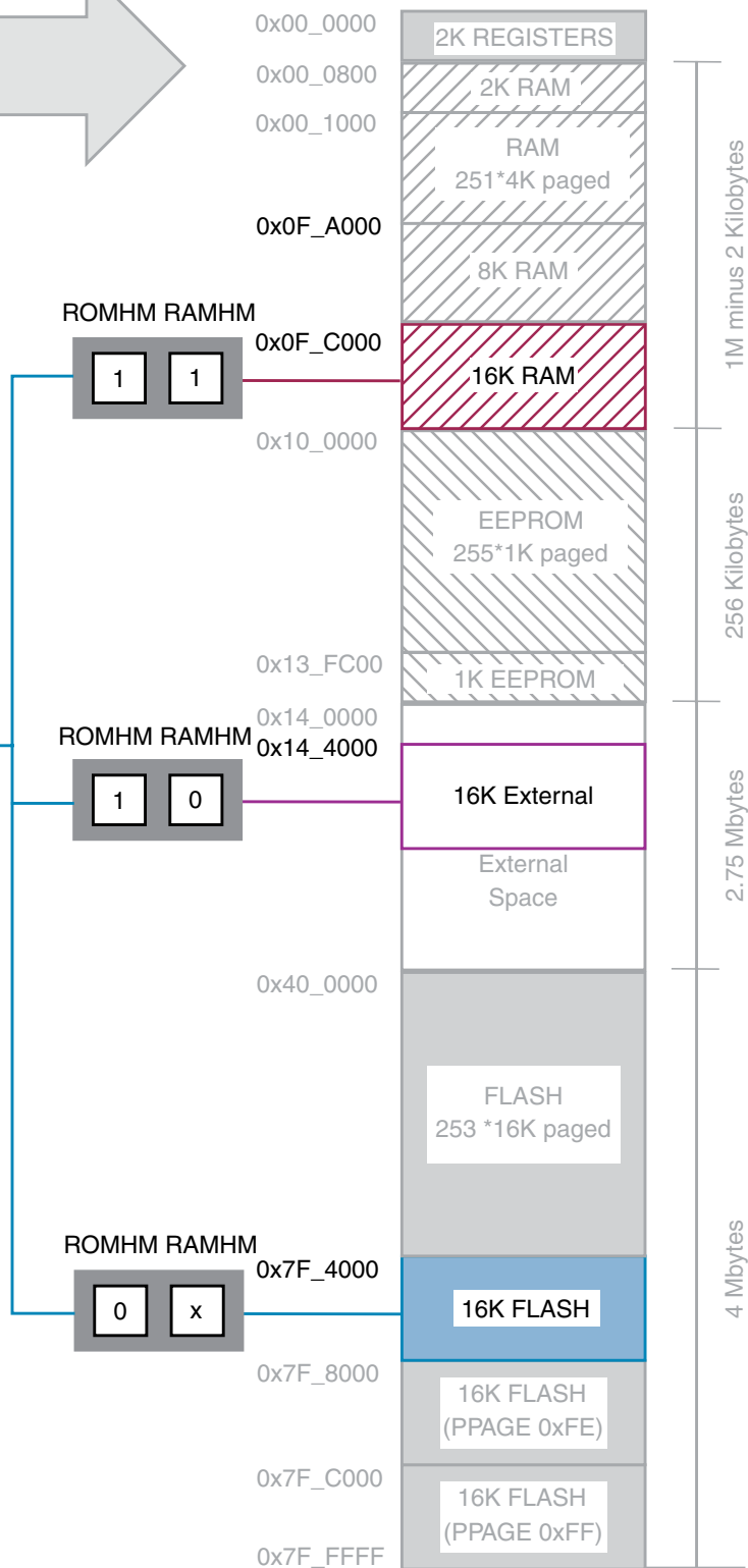
Figure 3-21. ROMHM, RAMHM Memory Configuration
