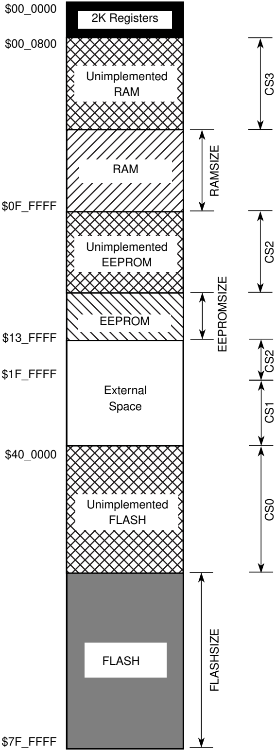
Figure 17-23. Local to Implemented Global Address Mapping (Without GPAGE)
